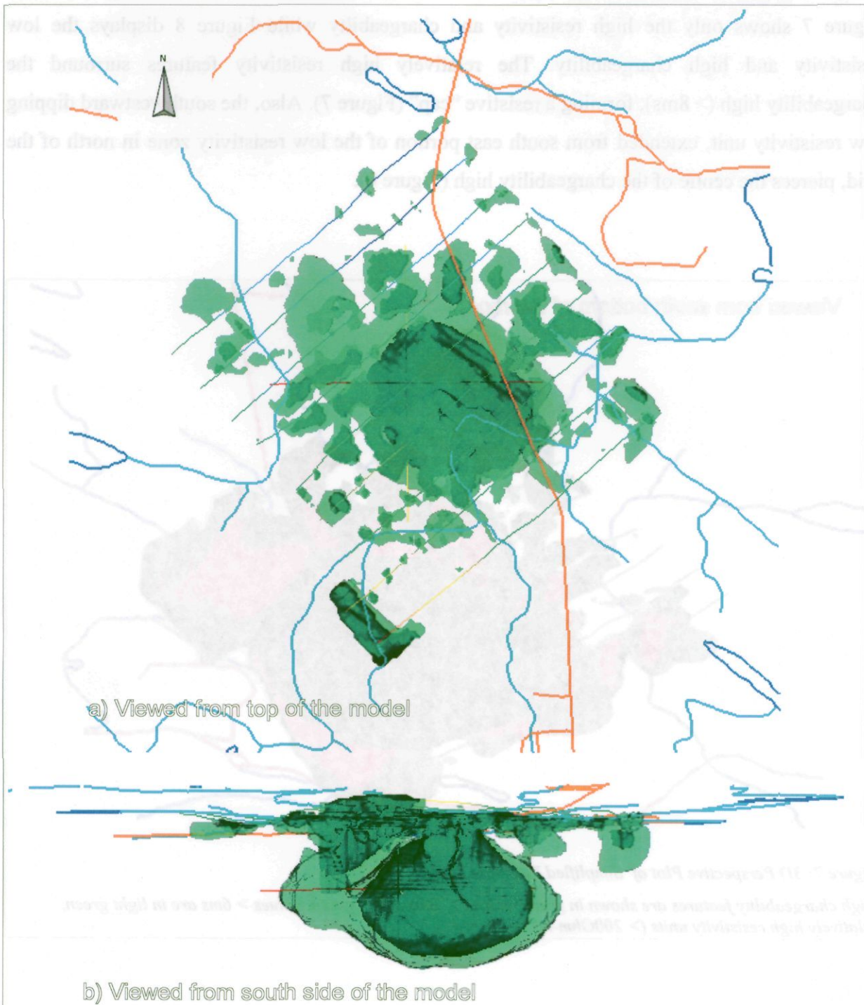
Figure 6: 3D Perspective Plots of Simplified Chargeability Inversion Model
