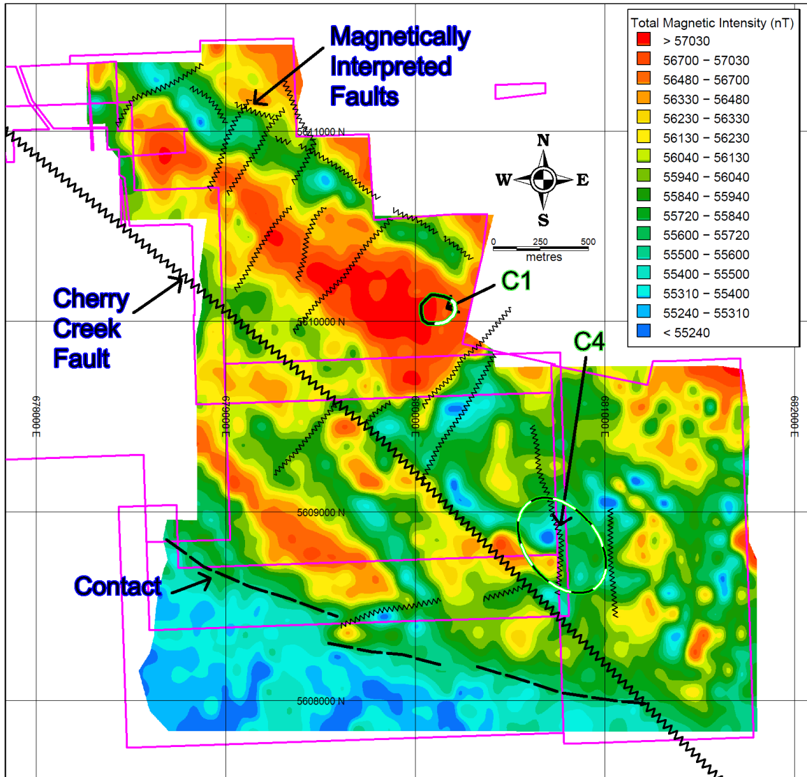
Figure 4: Total magnetic Field Intensity (Plate Mag-3) – interpreted linear features.
